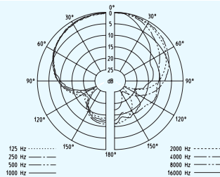
Polar diagram MMK 965-1 (super-cardioid)
