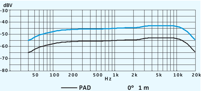
Frequency response curve MMK 965-1 (super-cardioid)
