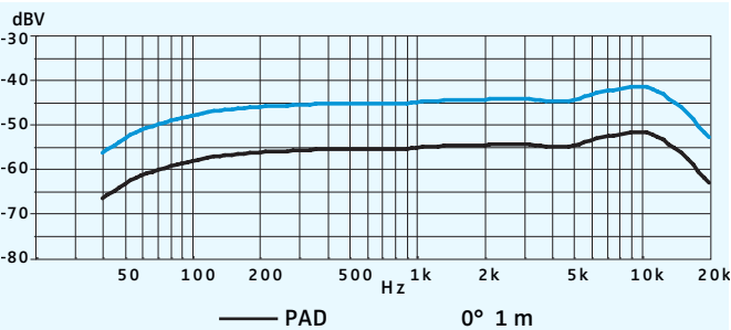
Frequency response curve MMK 965-1 (cardioid)
