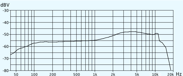
Frequency response curve MMD 945-1
