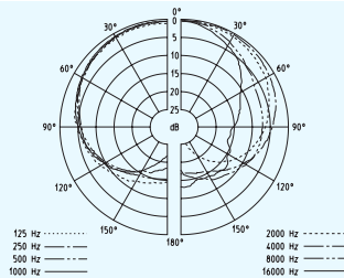
Polar diagram MMK 965-1 (cardioid)
