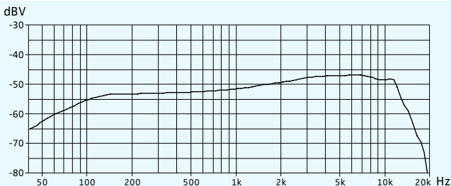
Frequency response curve MMD 935-1
